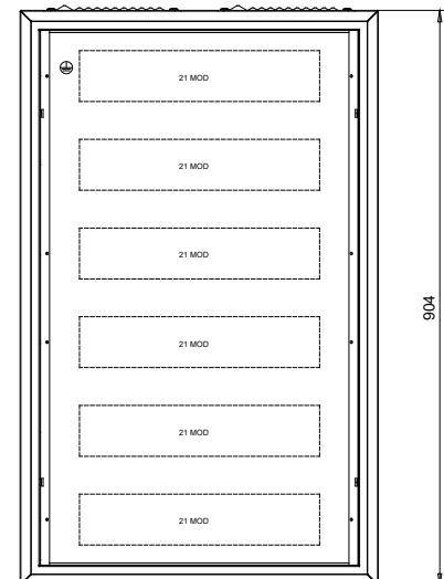
VARMA RX-126B 33 001 51
